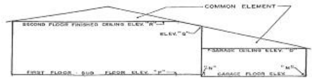
TYPICAL UNIT CROSS-SECTION A-A SCALE: 1" = 10'
